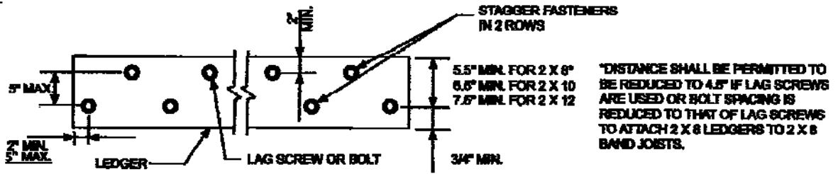
FIGURE R507.2.1(1) PLACEMENT OF LAG SCREWS AND BOLTS IN LEDGERS History: 2015 AACs.
