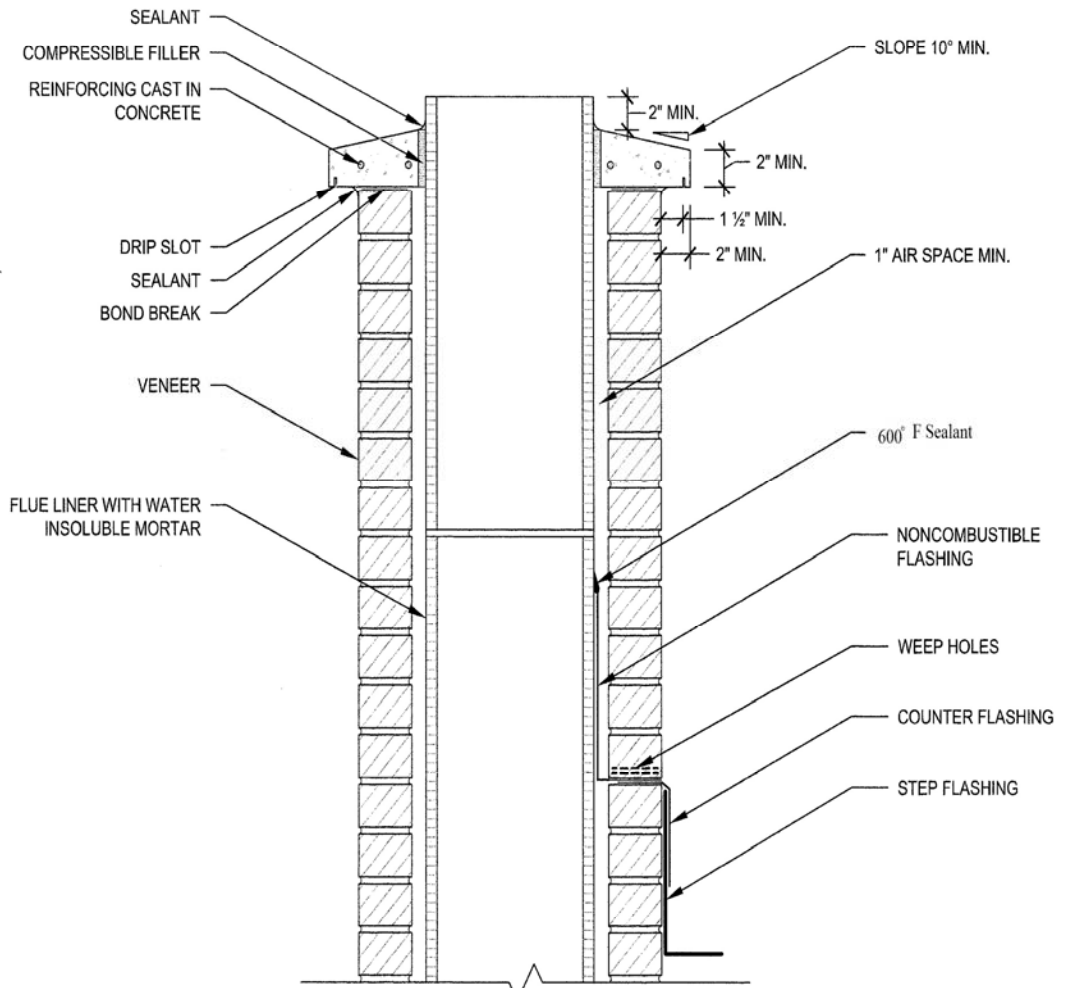
FIGURE R1003.9.1 (1)
