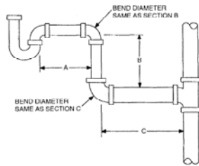
FIGURE P3105.4 VERTICAL LEG FIXTURE DRAIN SCHEMATIC
