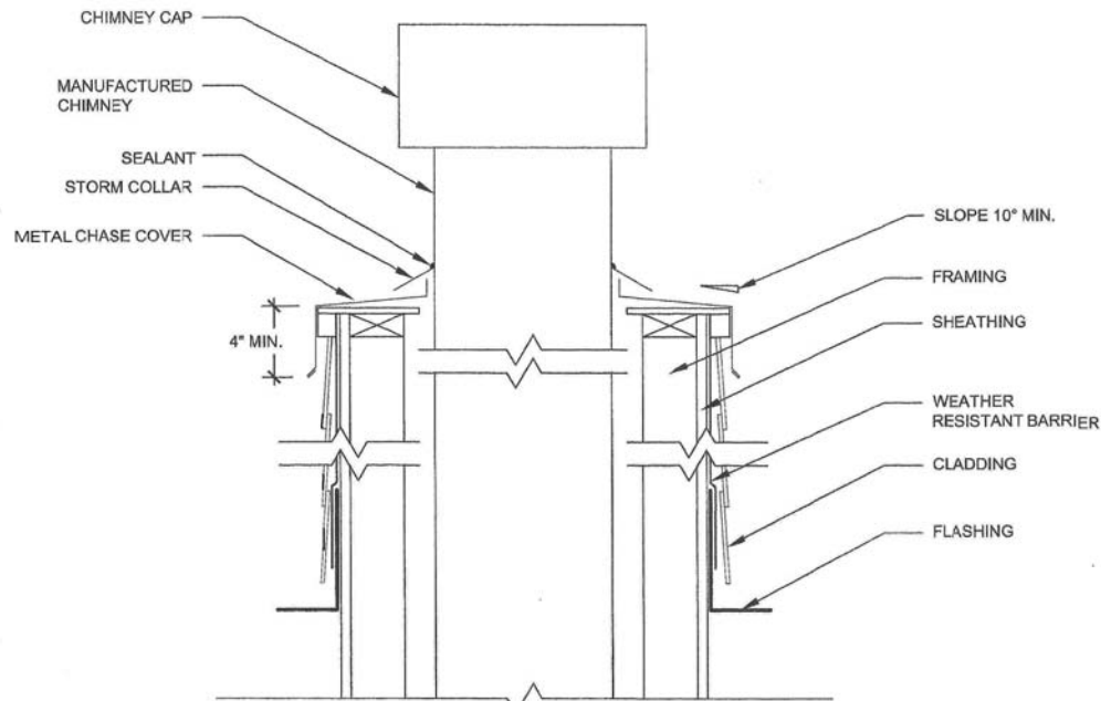
FIGURE R1003.9.1 (2)
